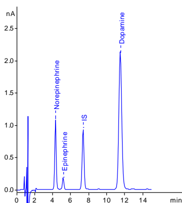
Fig. 2. Analysis of 20 µL ClinCal® urine calibrator. Concentration of catecholamines in the calibrator sample: 123 µg/L NA, 29.5 µg/L A and 227 µg/L Dopamine.
