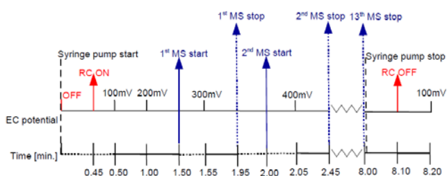
Fig. 6. Operation principle of mass voltammogram acquisition. RC – ReactorCell; MS – mass spectrometer. Details see text.
