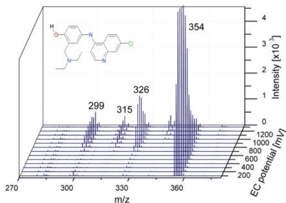
Fig. 5. Example of a mass voltammogram of Amodiaquine. Ion abundance versus m/z as a function of EC potential.
