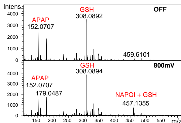
Fig. 9. Mass spectra acquired for ReactorCell OFF ( t = 3 min after start MS acquisition) and EC=800mV ( t=7 min), respectively. The mass spectra are extracted from the experiment showed in figure 8.
