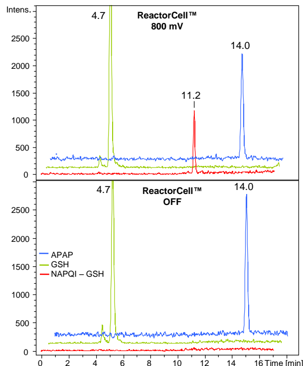
Fig. 1. Automated generation of phase I and II metabolites of APAP using the ROXY™ EC/LC system: with Reactor Cell™ ON (top) immediate formation of the NAPQI—GSH conjugate (phase II reaction) is observed (red).
