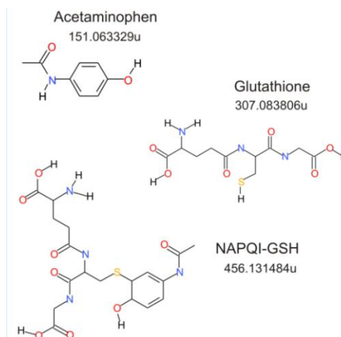
Fig. 2. Structures and monoisotopic masses of acetaminophen, glutathione and conjugate of the reactive metabolite of acetaminophen (NAPQI-GSH).
