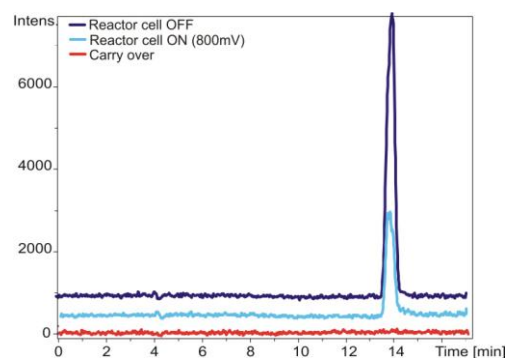
Fig. 5. Extracted ion chromatograms (EIC) of APAP (m/z= 152 Th), eluted in 14 min. 65% conversion of the APAP is observed with ReactorCell™ ON (800mV; light blue). Dark blue trace corresponds to control measurements with ReactorCell™ OFF. Red trace is a mobile phase injection
