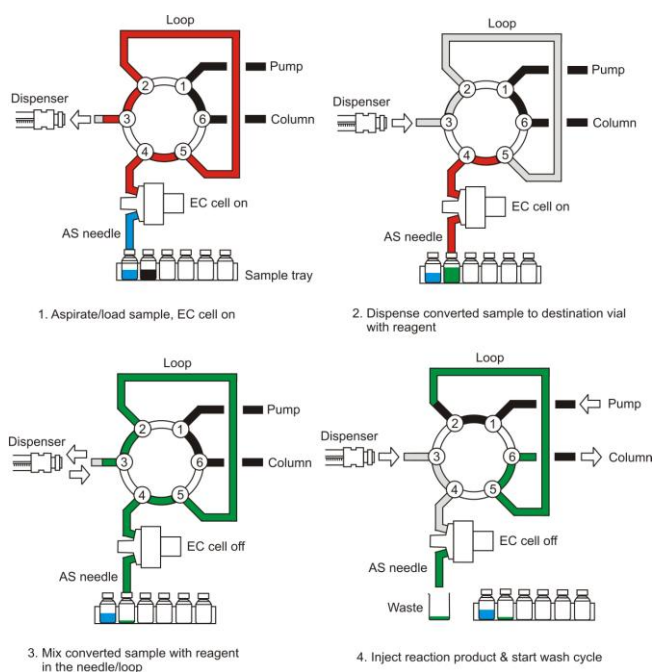
Fig. 6. Simplified schematic representation of the automated Phase II injection routine. Blue: sample, red: oxidized sample, black: reagent and green: oxidized sample mixed with reagent.
