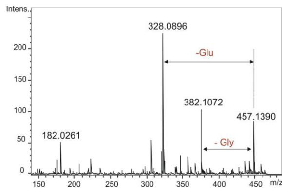
Fig. 8. Fragmentation spectrum (MS/MS) of conjugation product.
