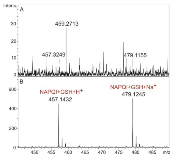
Fig. 7. Result of conjugation of phase I metabolite of acetaminophen (NAPQI) and GSH. (A.) ReactorCell OFF, (B.) ReactorCell EC = 800mV.
