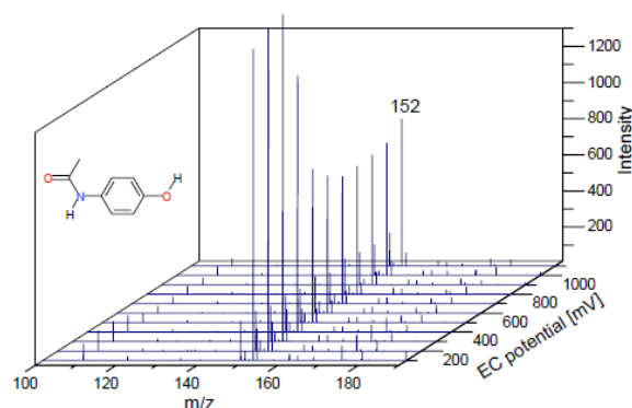
Fig. 4. Mass voltammogram of acetaminophen.
