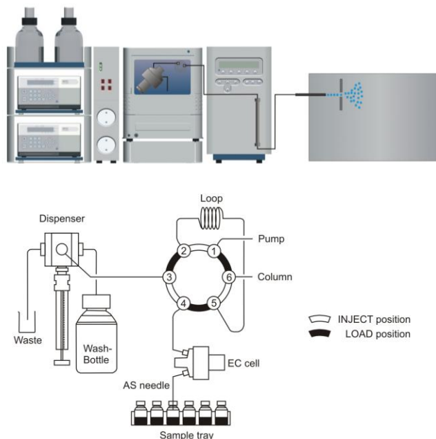
Fig. 3. Top : ROXY™ EC/LC System including ReactorCell™ integrated in the AS110 autosampler flow path. Bottom : Detailed lay-out of autosampler flow path with 6-port injection valve and ReactorCell™
