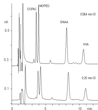
Fig. 3 Dispersion by tubing. 60 \mu\text{m} vs 250 \mu\text{m} tubing.
