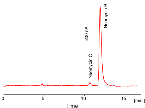
Fig. 3. Example chromatogram of a 75 \mu g/mL Framycetin sulphate reference standard solution (EP BP190–F67029), 10 \mu L injected (Note that chromatogram 1b was recorded with slightly different LC conditions as 1a).
