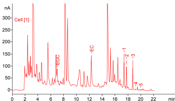
Fig. 4: Chromatogram of 10X diluted Santa Digna cabernet sauvignon (1), 2003, Chile; 1= Myricetin, 2= trans-Resveratrol, 3= Quercetin, 4= cis-Resveratrol and 5= Keampferol
