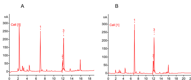
Fig. 5A: Analysis of 50X diluted Lipton green ice tea, Unilever, 1= EGC, 2= EC, 3=EGCG and (5B) 50X diluted green tea, Pickwick; 1= EGC, 2= EC and 3= EGCG.
