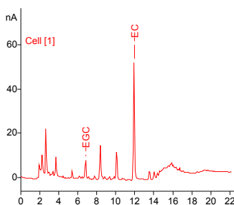
Fig. 6: Chromatogram of Milk chocolate (Trésor, the Convenience company), extracted and diluted 50X; 1= EGC, 2= EC
